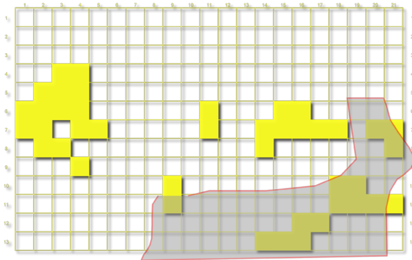
Figure 13: Estimated Location of Surficial Aquifer
