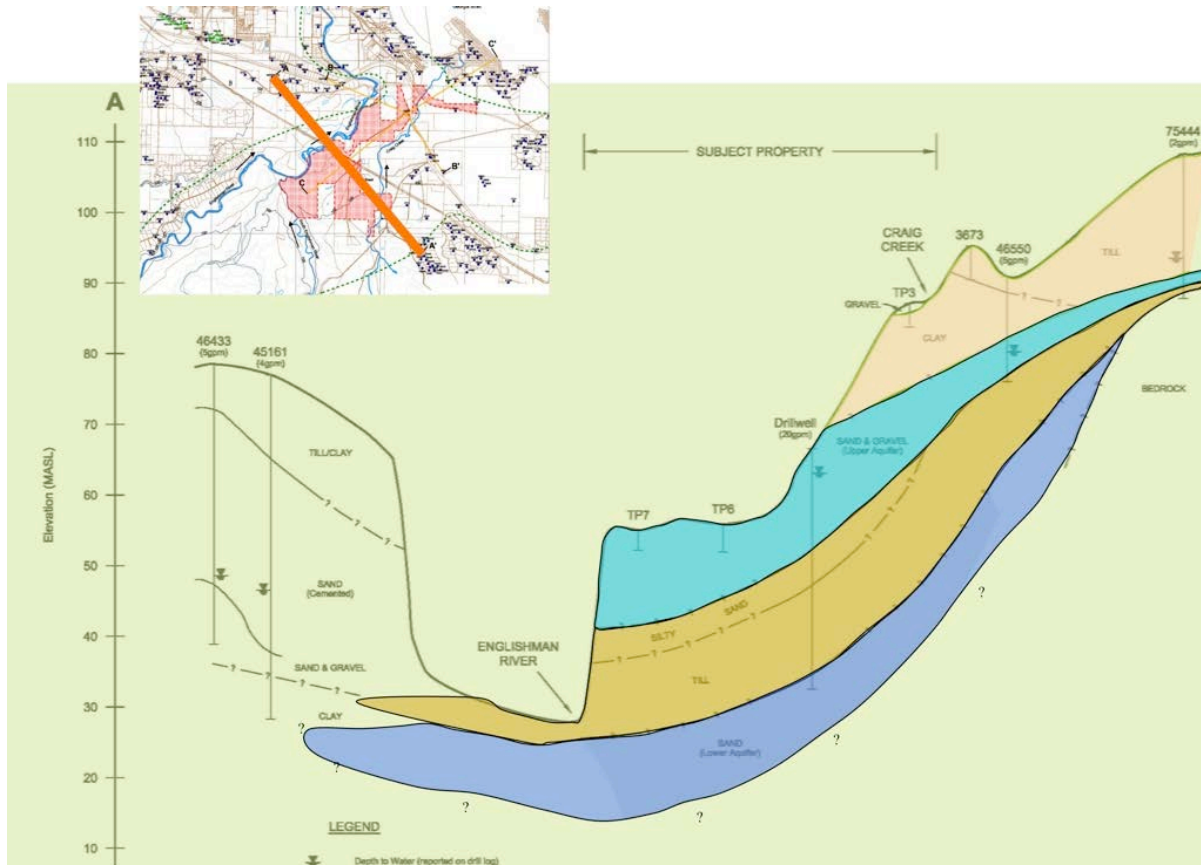
Figure 16: NW-SE Cross-Section Through River's Edge Subdivision
