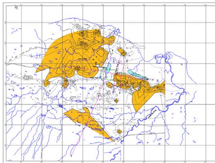
Figure 15: Estimated Location of Shallow Till and Reported Historical Artesian Conditions
