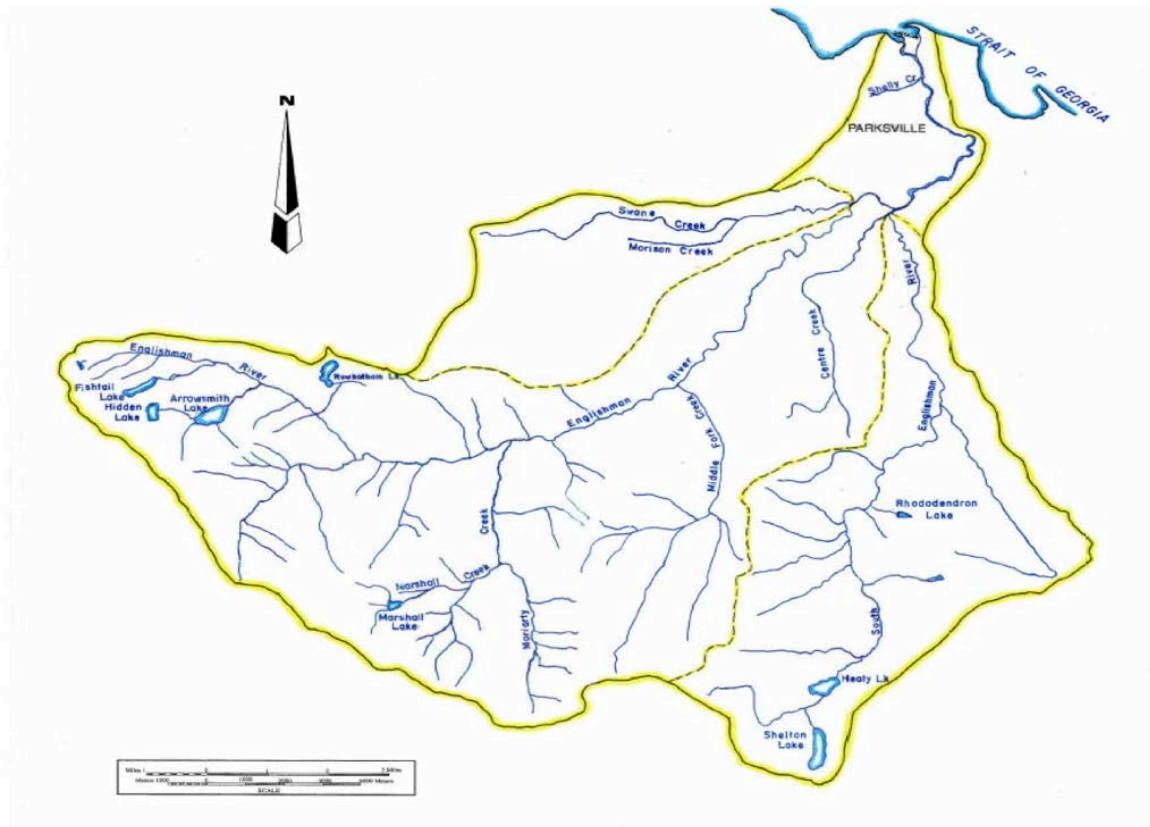
Figure 3: Englishman River Drainage System
