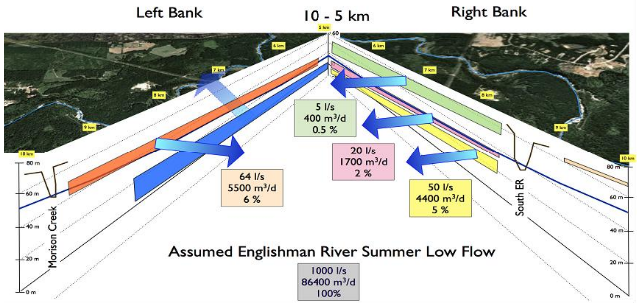
Estimated Groundwater Flux to Englishman River from Overburden Aquifers
